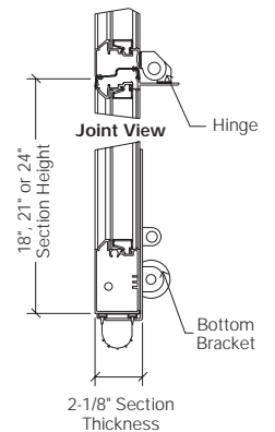
SECTION A-A BOTTOM BRACKET VIEW
