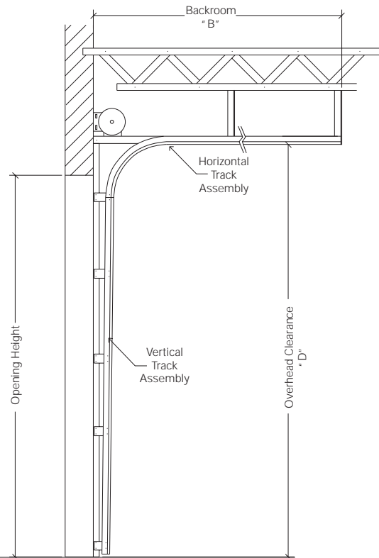
STANDARD LIFT TRACK
