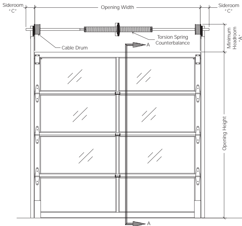
INTERIOR ELEVATION
